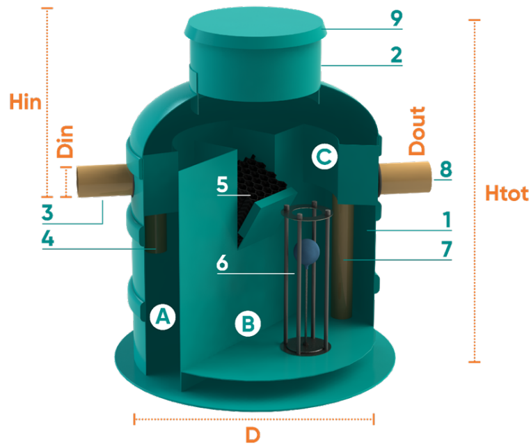
Fig. 1 Oil/Water Separator Vodaland OilBase 100 with Bypass
